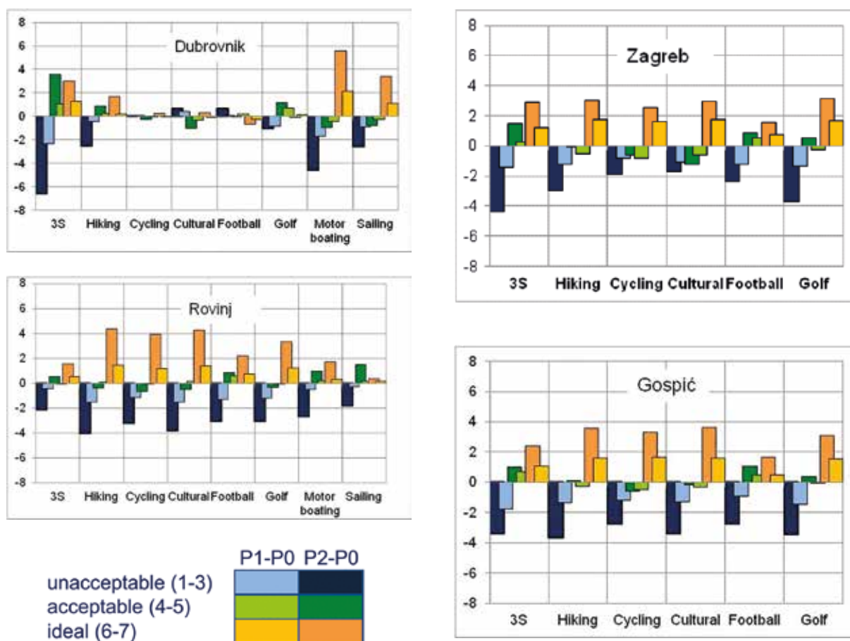
Figure 1: Annual differences between occurrences of unacceptable, acceptable and ideal climate conditions for different types of tourism according to CIT between future (P1 for 2011-2040, P2 for 2041-2070) and present (P0) climates at southern (Dubrovnik) and northern (Rovinj) Adriatic and continental lowland (Zagreb) and highland (Gospić)
