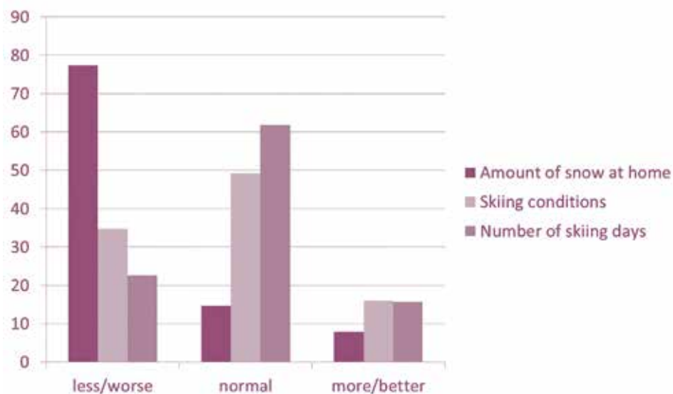
Figure 1: Perceived snow conditions at home and during skiing trips and change of skiing days in the 2013/14 season
