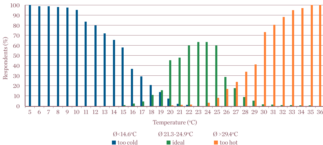
Figure 1: Temperature preferences and thresholds for mountain summer tourism (too cold: n=712; ideal: n=730; too hot: n=716)
