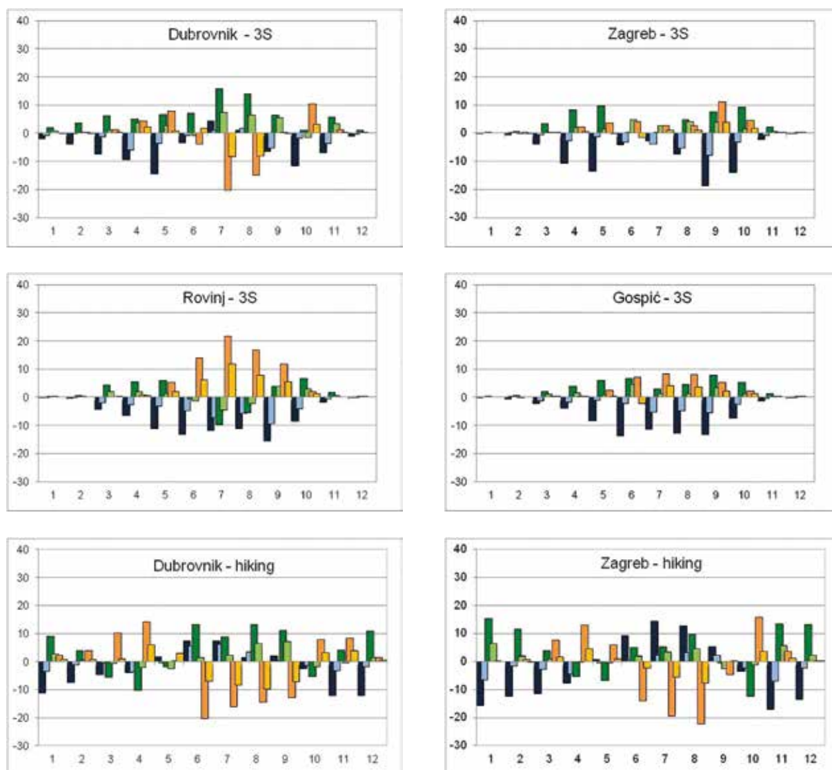
Figure 2: Differences between occurrences of unacceptable, acceptable and ideal climate conditions for 3S tourism (above) and hiking (below) according to CIT between future (P1 for 2011-2040, P2 for 2041-2070) and present (P0) climates at southern (Dubrovnik) and northern (Rovinj) Adriatic and continental lowland (Zagreb) and highland (Gospić)
