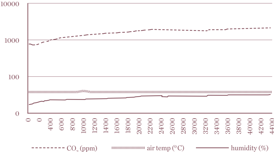
Figure 1: Carbon dioxide, air temperature and humidity while driving the car
