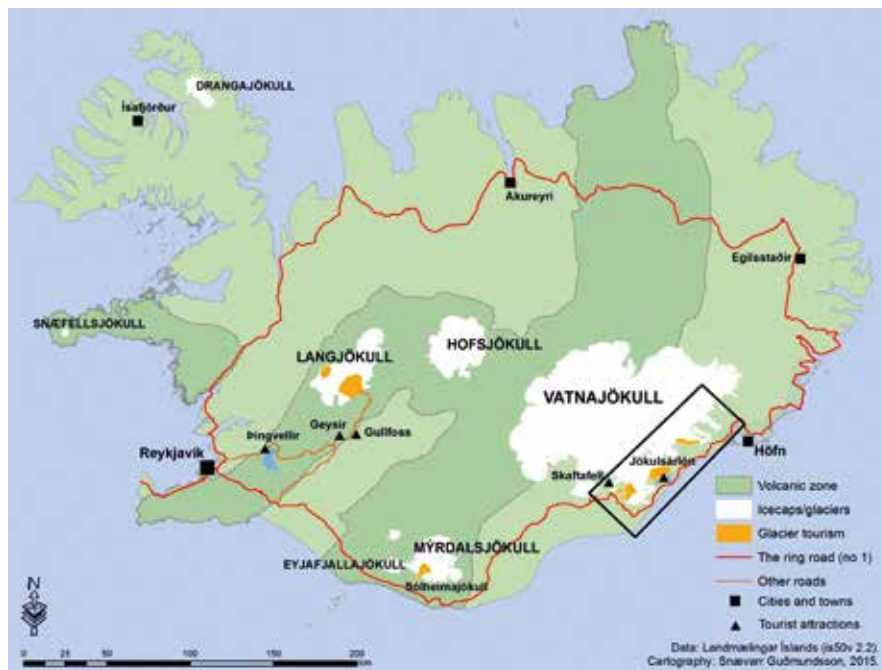
Figure 1: Map of glacier sites in Iceland and the study area, the Vatnajökull region (rectangle)
