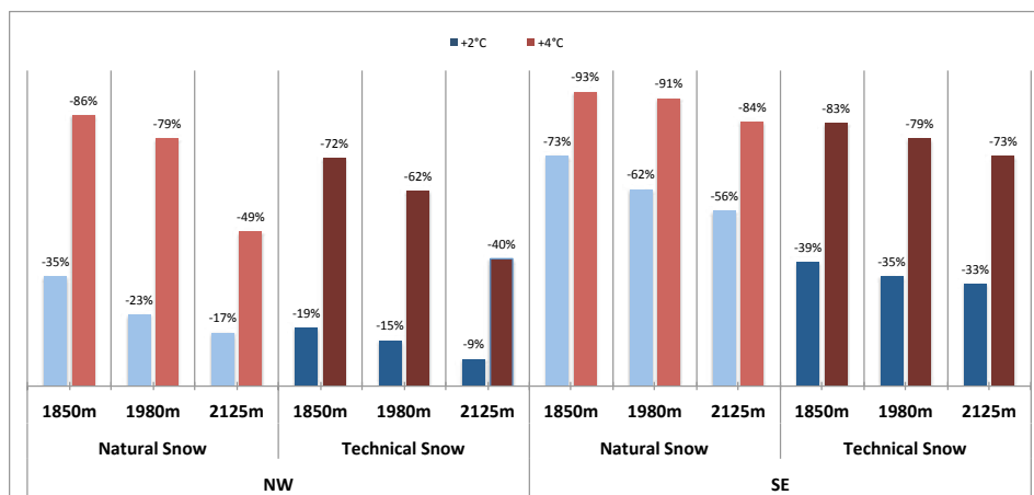
Figure 4: Decrease in the number of days with at least 30 cm snow (reliability criteria) based on altitude and aspect (NW and SE) in two different climate scenarios (+2°C and +4°C), analyzing the effect of grooming and snowmaking (technical snow) in a ski resort of the central part of the Spanish Pyrenees
