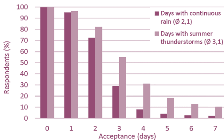
Figure 2: Acceptance of days with summer thunderstorms (n=699) and days with continuous rain (n=716)
