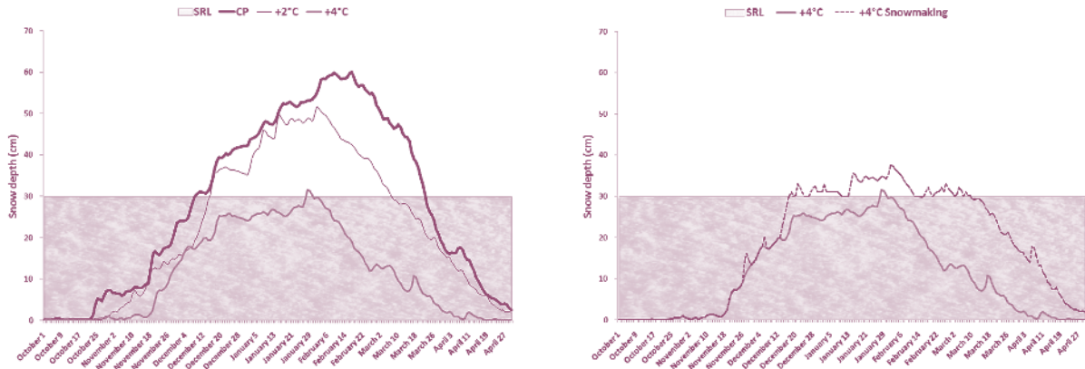
Figure 2: Projected changes on the natural snowpack at the mean elevation of a ski resort in the central-eastern part of the French Pyrenees in a medium (+2°C increase of the mean winter temperature) and high-climate change scenario (+4°C)
