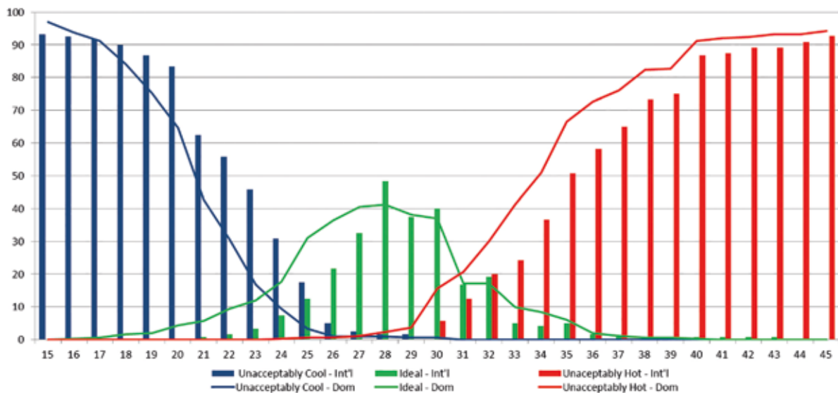
Figure 1: Temperature preferences and thresholds for Canadian beach tourists travelling internationally and domestically
