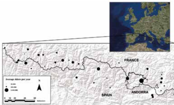
Figure 1: The Pyrenees region and the location of the alpine ski resorts (The size of the dots represents the average of the yearly attendance from 2009 to 2012.)
