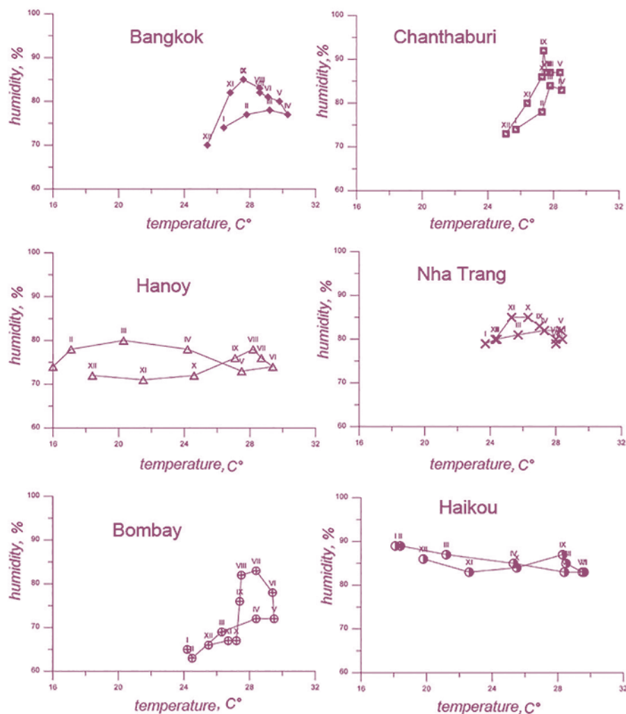
Figure 2: Climatograms of temperature and humidity conditions of the individual stations of the Southern and Southeastern Asian countries
