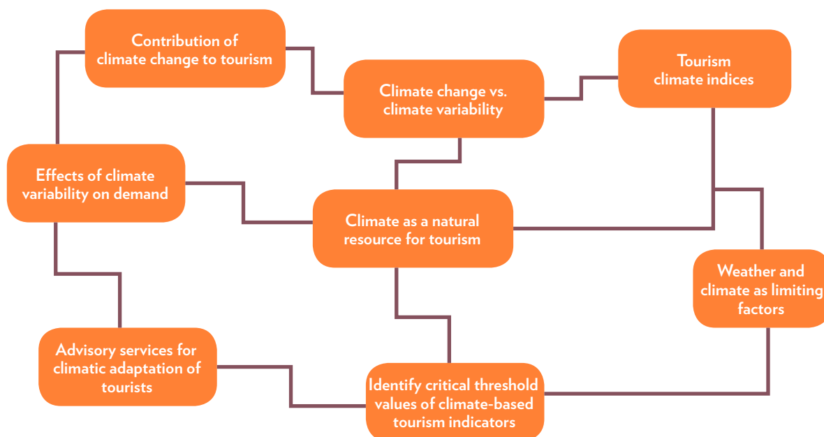
Figure 1: Current climate-tourism relationships: themes and issues
