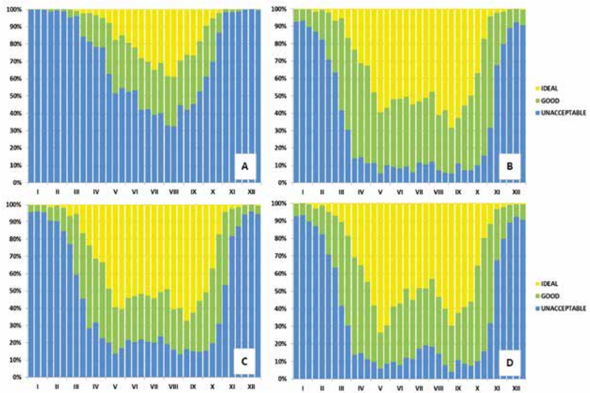
Figure 1: Average 10-day frequencies of CIT categories in Siófok for 1961-1990
