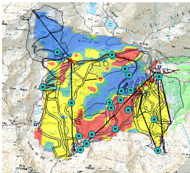
Figure 4: Decrease in the number of days with at least 30 cm snow (reliability criteria) based on altitude and aspect (NW and SE) in two different climate scenarios (+2°C and +4°C), analyzing the effect of grooming and snowmaking (technical snow) in a ski resort of the central part of the Spanish Pyrenees
