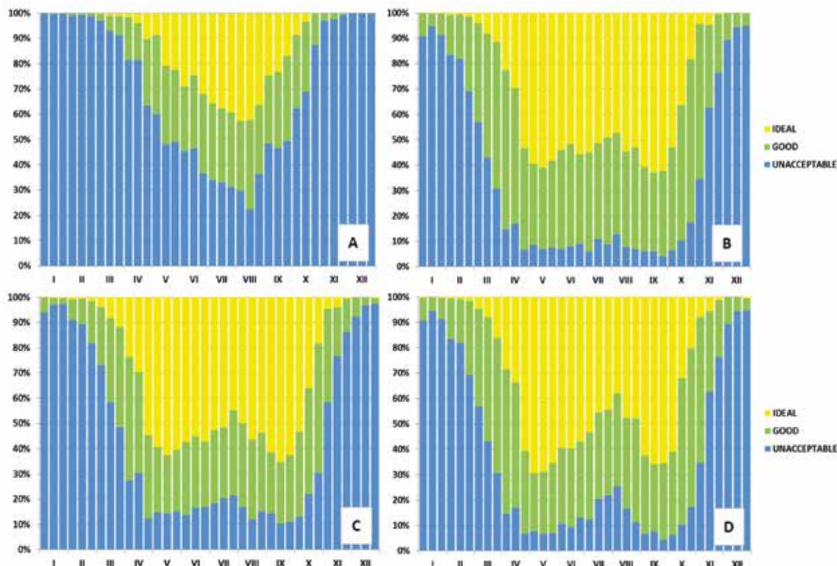
Figure 2: Average 10-day frequencies of CIT categories in Siófok for 1981-2010 A-beach; B-cultural; C-cycling; D-hiking
